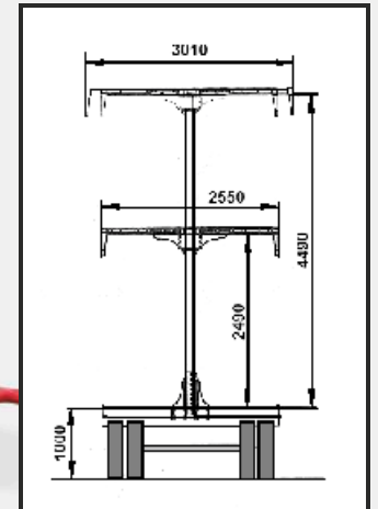
Round bales compression side extension.
